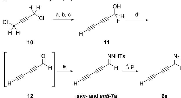
Scheme 4. Synthesis of 1-Diazo-2,4-pentadiyne ( 6a ) from 1,4-Dichloro-2-butyne ( 10 ) a
